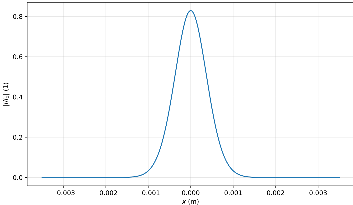
Intensity profile I(x, y = 0, z = 1.194m)/I_0 , P_{in}=0.2P_{cr} , artificial time
